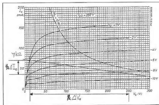
fig.23 Optimale belasting penthode.
